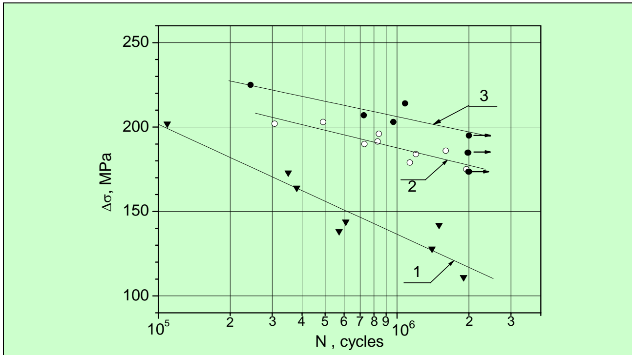
Fatigue curves of large-scale welded samples (transverse non-load-carrying attachment): 1 – in as welded condition, 2 – UP was applied before fatigue testing, 3 – UP was applied after fatigue loading with the number of cycles corresponding to 50% of expected fatigue life of samples in as-welded condition
